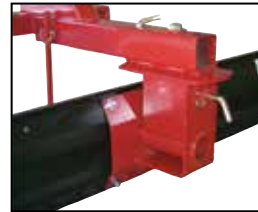
3-position tilt assembly
